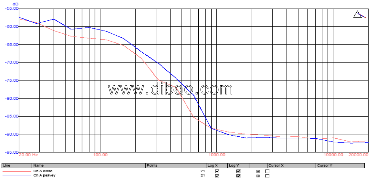
THD+N vs frequency
